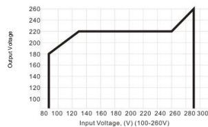
Input voltage & Output Voltage diagram
