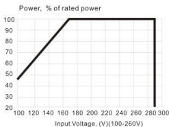
Loading Capability Diagram
