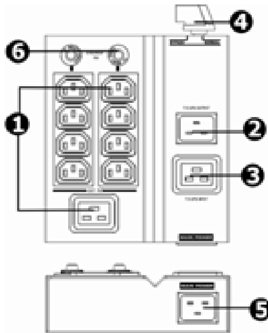
IEC outlets
