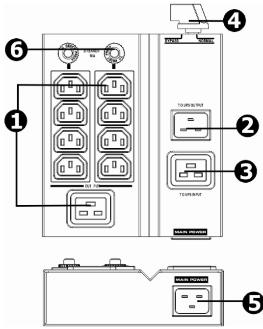
Prises IEC
