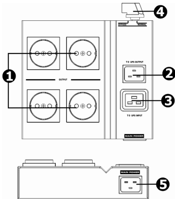
FR outlets
